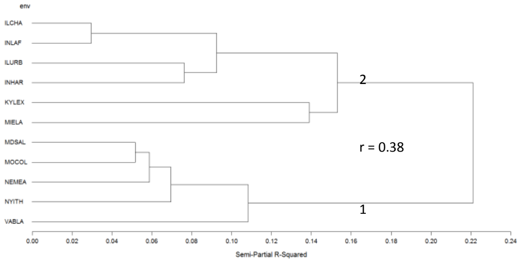
Figure 1. NUWWSN FHB Incidence Bi-plot from AMMI (PC1 versus PC2, entry numbers are shown) and clusters of environments using the G×E matrix and Ward's minimum variance
