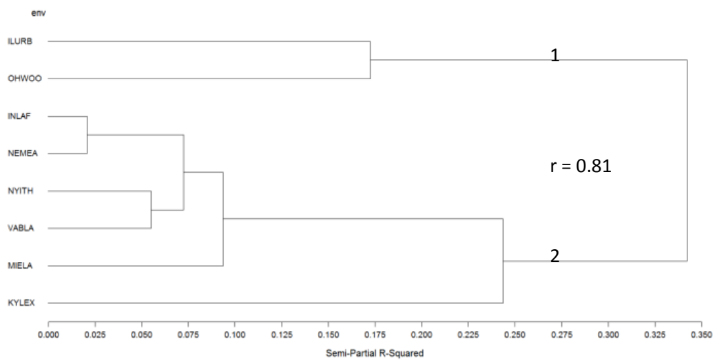
Figure 6. NUWWSN FHB DON Bi-plot from AMMI (PC1 versus PC2, entry numbers are shown) and clusters of environments using the Gx \epsilon matrix and Ward's minimum variance.
