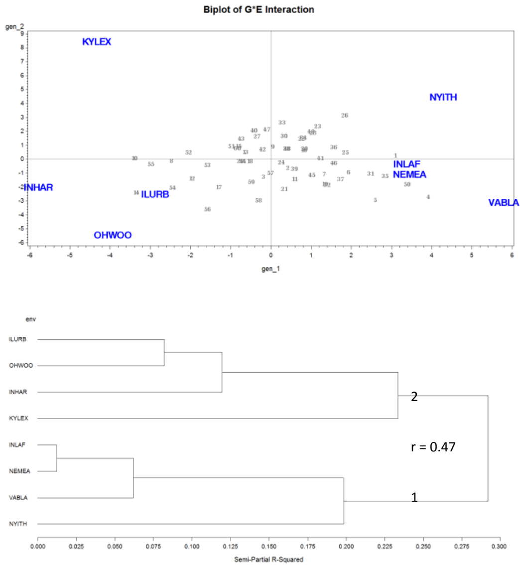
Figure 4. NUWWSN FHB FDK Bi-plot from AMMI (PC1 versus PC2, entry numbers are shown) and clusters of environments using the Gx E matrix and Ward's minimum variance.
