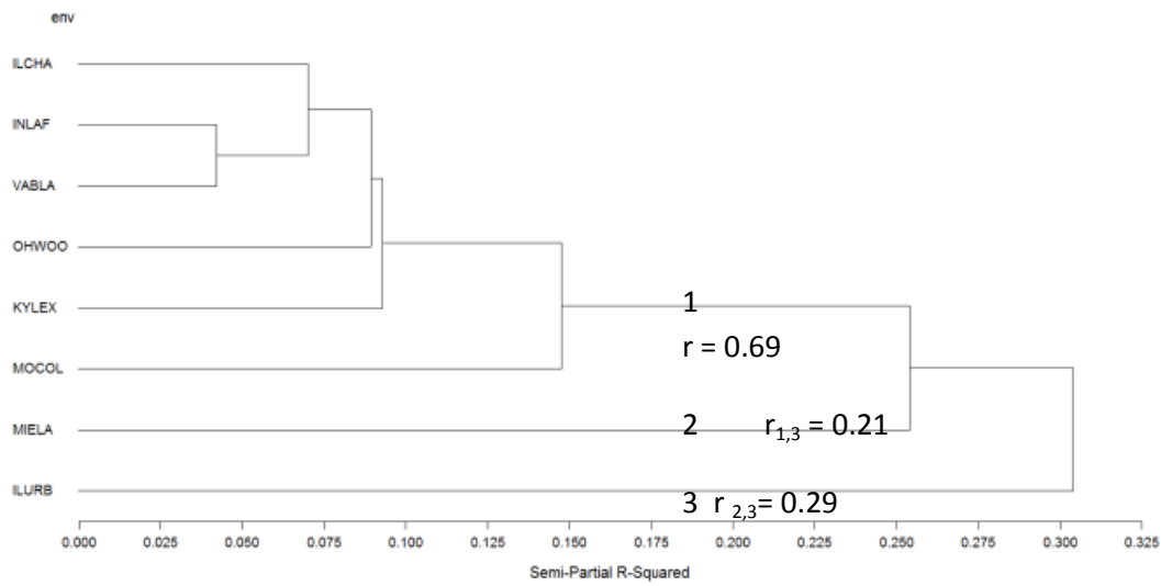
Figure 9. PNUWWSN FHB Index Bi-plot from AMMI (PC1 versus PC2, entry numbers are shown) and clusters of environments using the G x E matrix and Ward's minimum variance.
