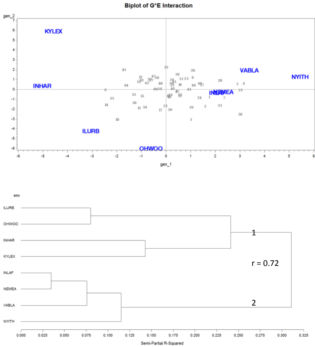
Figure 5. NUWWSN FHB ISK Bi-plot from AMMI (PC1 versus PC2, entry numbers are shown) and clusters of environments using the Gx \epsilon matrix and Ward's minimum variance.
