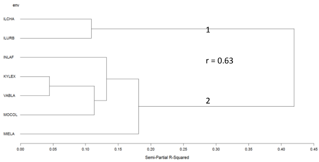
Figure 8. PNUWWSN FHB Severity Bi-plot from AMMI (PC1 versus PC2, entry numbers are shown) and clusters of environments using the G×E matrix and Ward's minimum variance.
