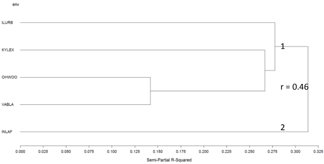
Figure 11. PNUWWSN FHB ISK Bi-plot from AMMI (PC1 versus PC2, entry numbers are shown) and clusters of environments using the G x E matrix and Ward's minimum variance.
